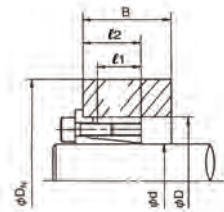
Fig. 3 (Short Hub without Guide) K_3=1.0
