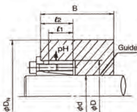
Fig. 1 (Long hub with guide) where B \geq 2\ell_1 K_3=0.8
