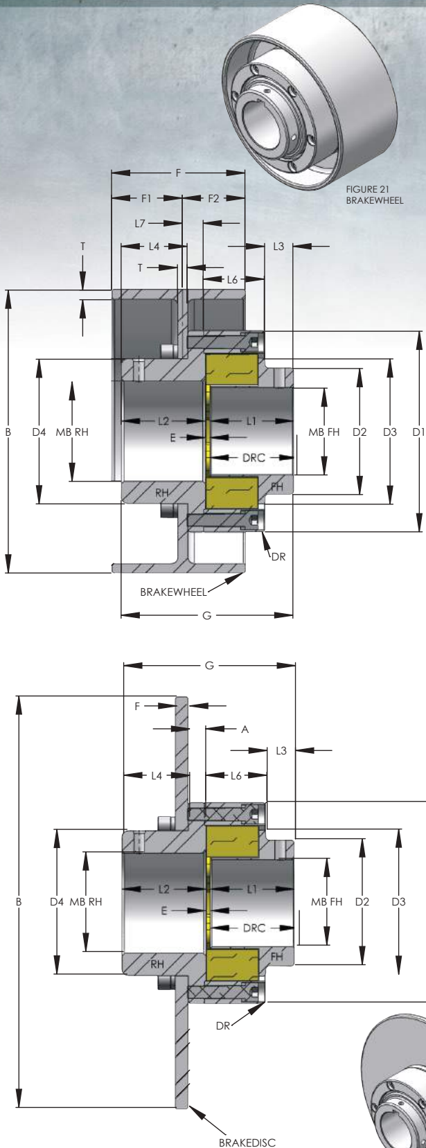
FIGURE 22 BRAKEDISC
