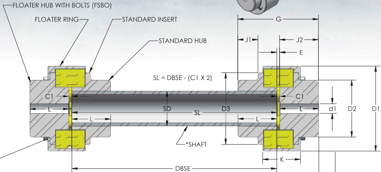
FIGURE 8 FLOATING SHAFT
