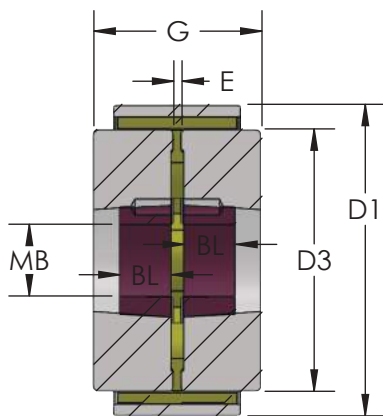
FIGURE 11 INTERNAL TAPER-LOCK
