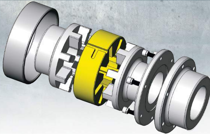
FIGURE 29 SPACER
