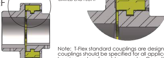
FIGURE 14 LIMITED END FLOAT
