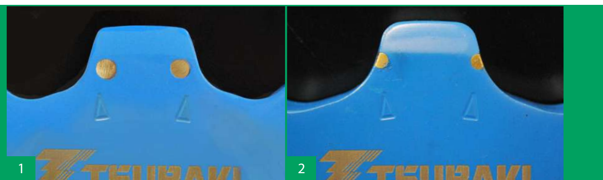
Figure 2 – Comparison – New (1) vs. Worn Sprocket (2)
