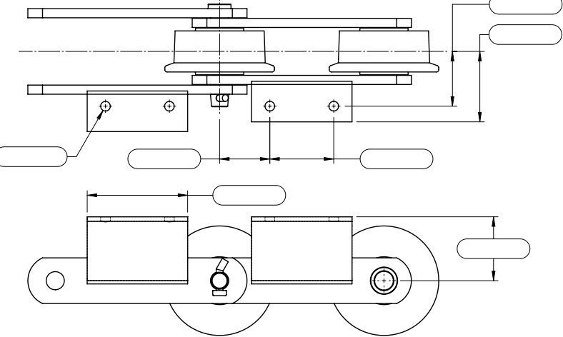
Angled Steel A2 Attachment Form
