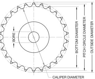
Measuring sprocket outside diameter
