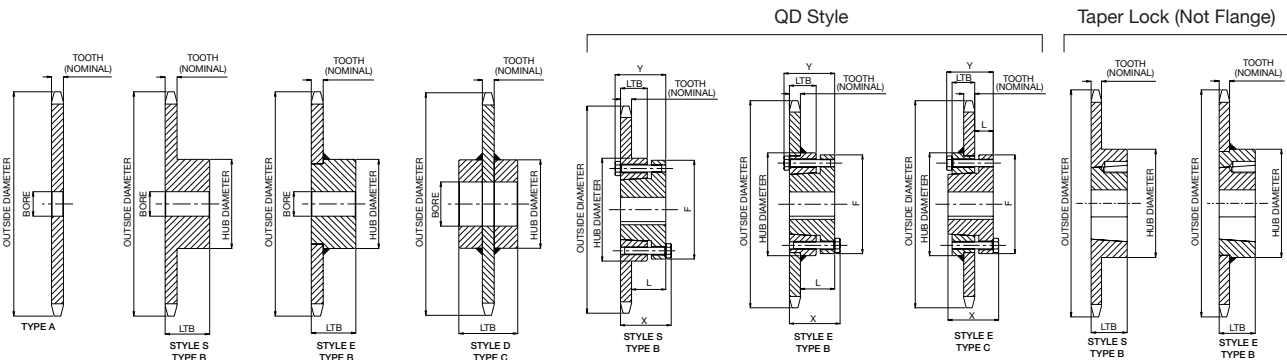
Stock sprocket hub styles
