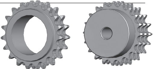
Multiple-Strand sprockets
