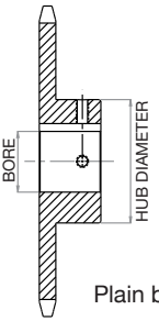
Maximum bore diameter and thru bore
