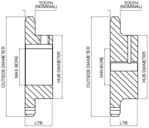
Maximum bore diameter and thru bore
