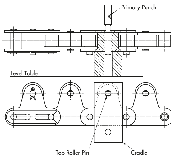
Figure 16: Removing Top Roller Pins
