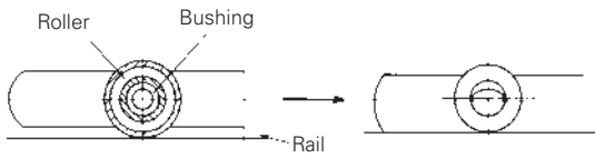
Figure 15-1: Roller Wear
