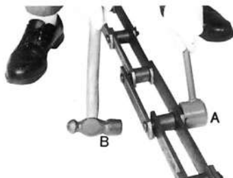
Figure 11-2: Putting on the Link Plate
