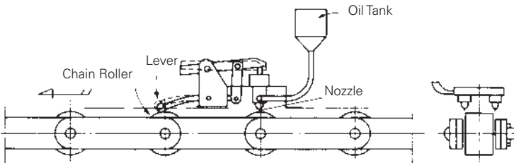
Figure 13-2: Automatic Drip Lubrication
