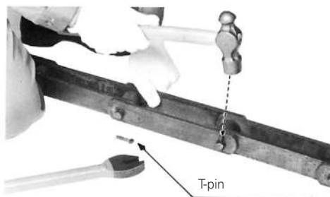
Figure 12-1: Removing the T-pins or Cotter Pins
