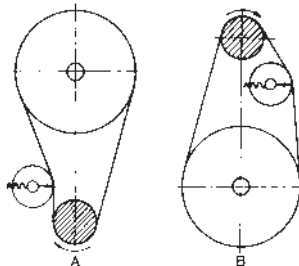
Figure 8-5: Vertical Centerlines
