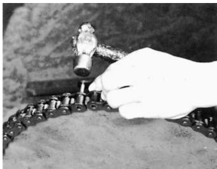
Figure 3-1: Connecting RS Roller Chain on a Sprocket
