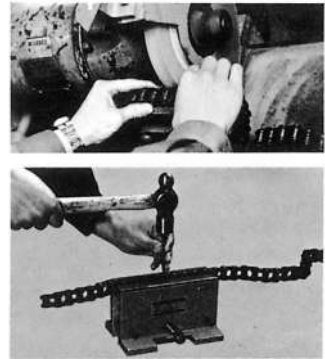
Figure 4-1: Disconnecting RS Roller Chain
