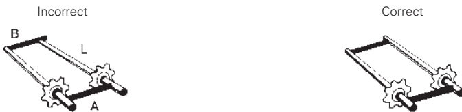
Figure 6-2: Shaft Parallelism
