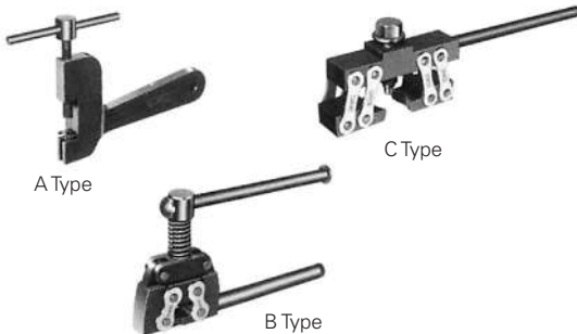
Figure 4-4: Chain Breaker Types
