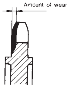
Figure 15-8: Sprocket Tooth Wear
