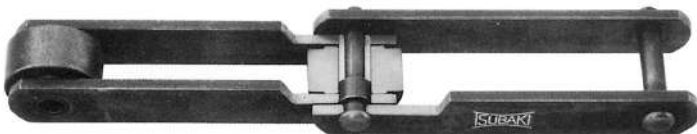
Figure 1-2: RF Conveyor Chain Construction
